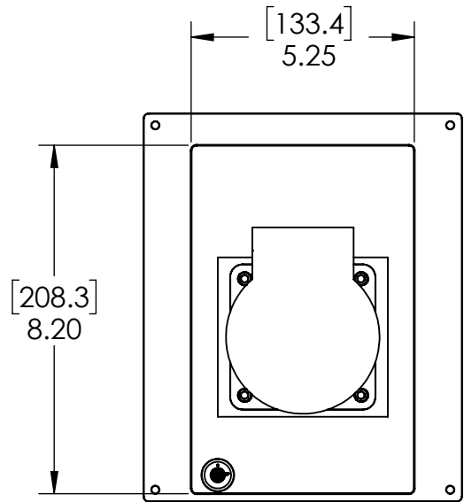
PANEL CUTOUT
