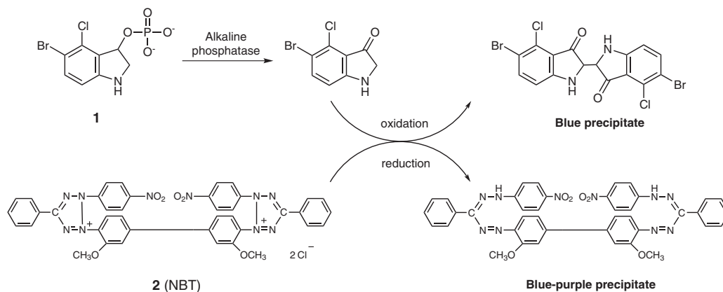
Chromogenic reaction of 1 / 2 by alkaline phosphatase.
