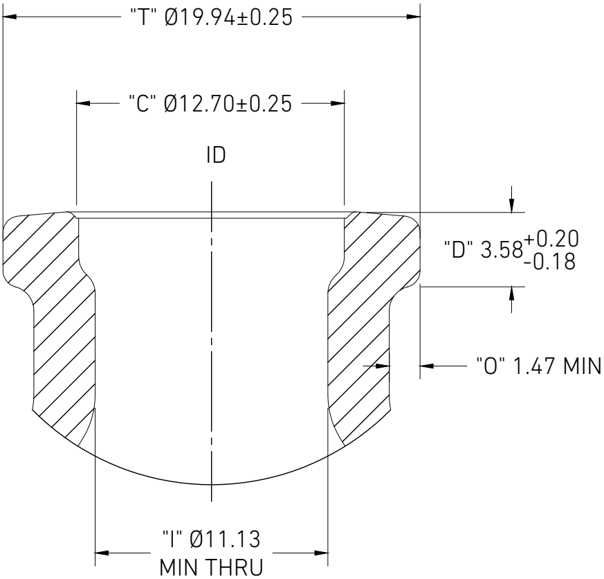
FINISH DETAIL SCALE 4 : 1
