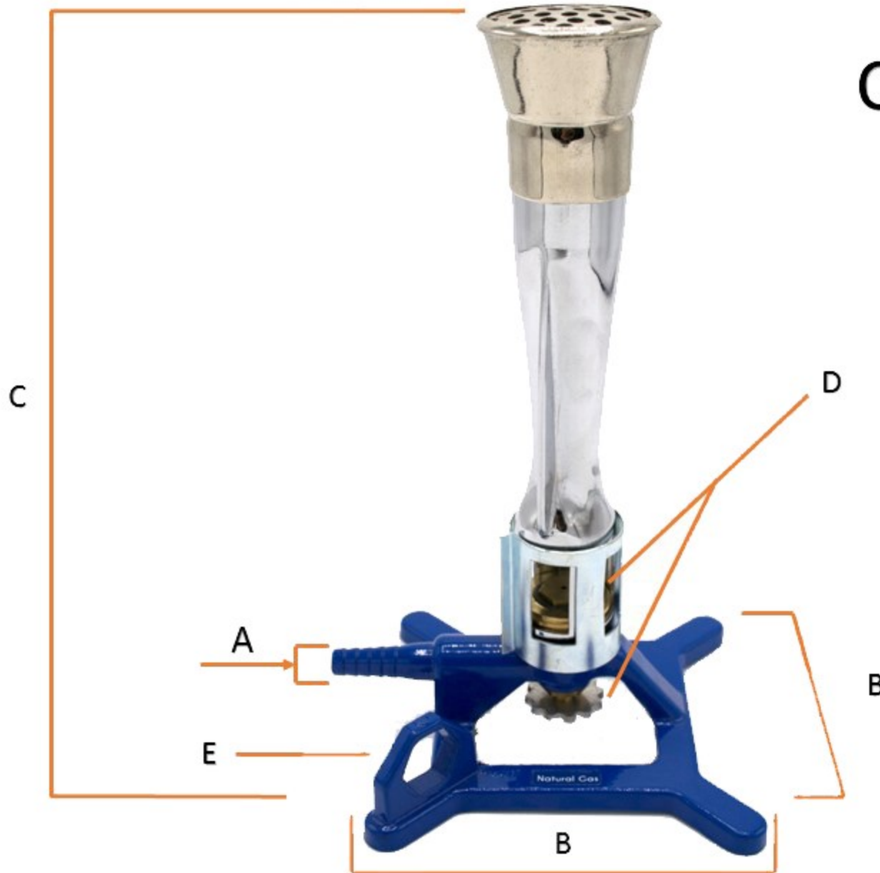
Eisco Labs NEXTGEN Meker Bunsen Burner, StabiliBase Anti-Tip Design with Handle, for use with Natural Gas
