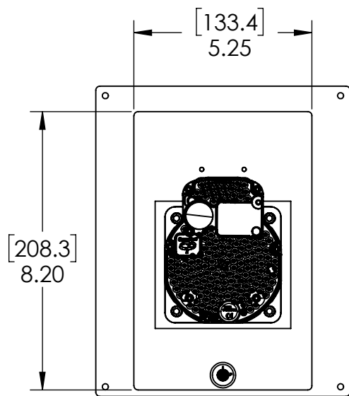
PANEL CUTOUT
