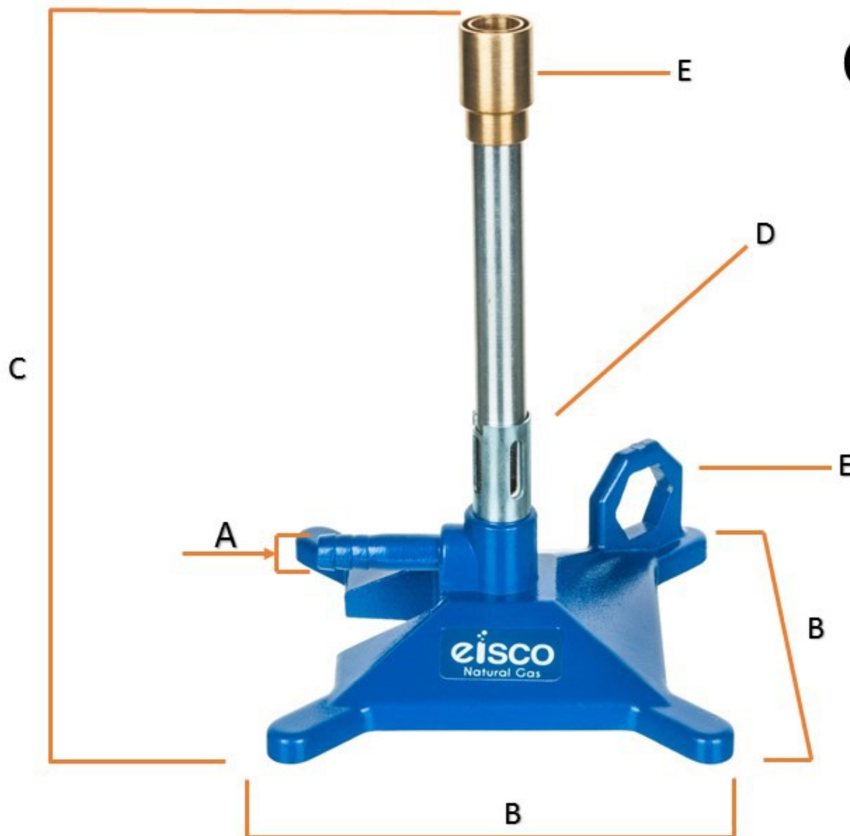
Eisco Labs NEXTGEN Bunsen Burner, Stabilibase Anti-Tip Design with Handle, for use with Natural gas
