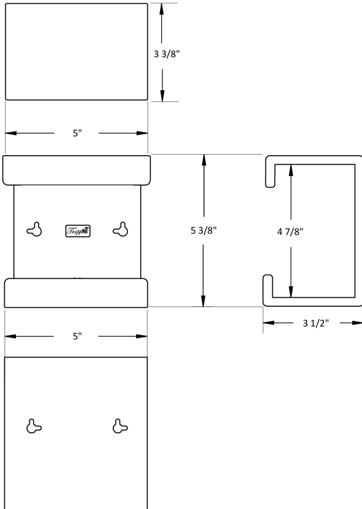
Part No: 50008 Small Kimwipe Holder with Keyholes
