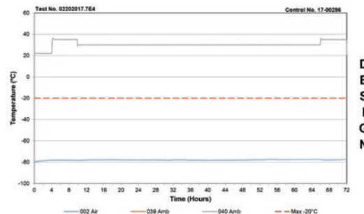
Sonoco ThermoSafe Model 89496-762 ISTA 7D Summer Ambient Profile
