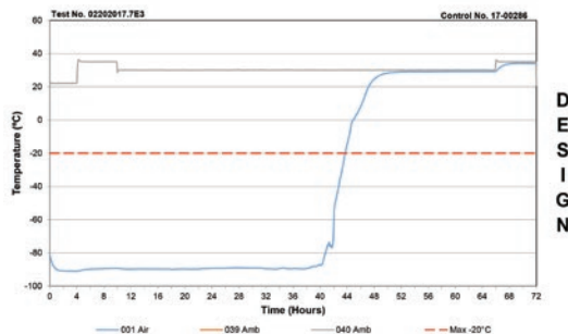
Sonoco ThermoSafe Model 95041-883 ISTA 7D Summer Ambient Profile
