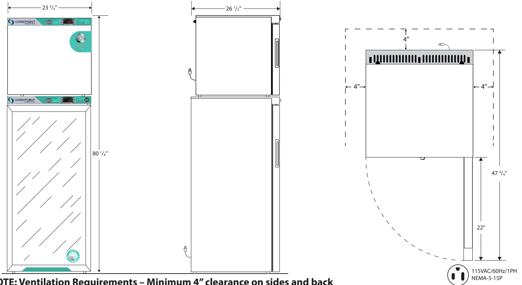
Top View
