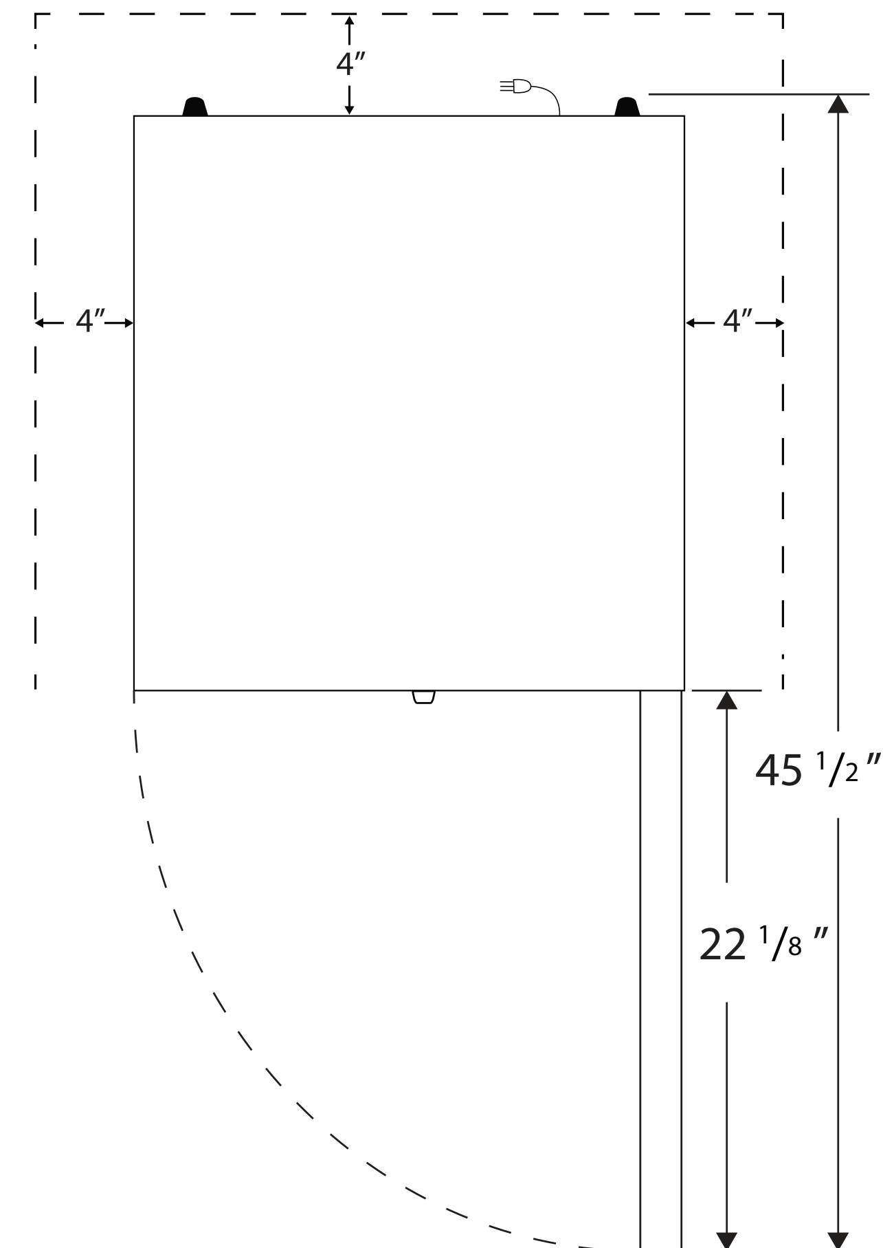
Top View
