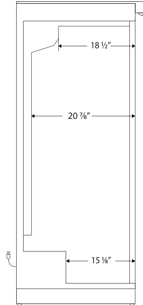
Side View
