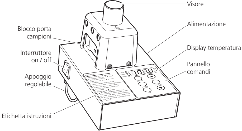
MP-200D Fascia
