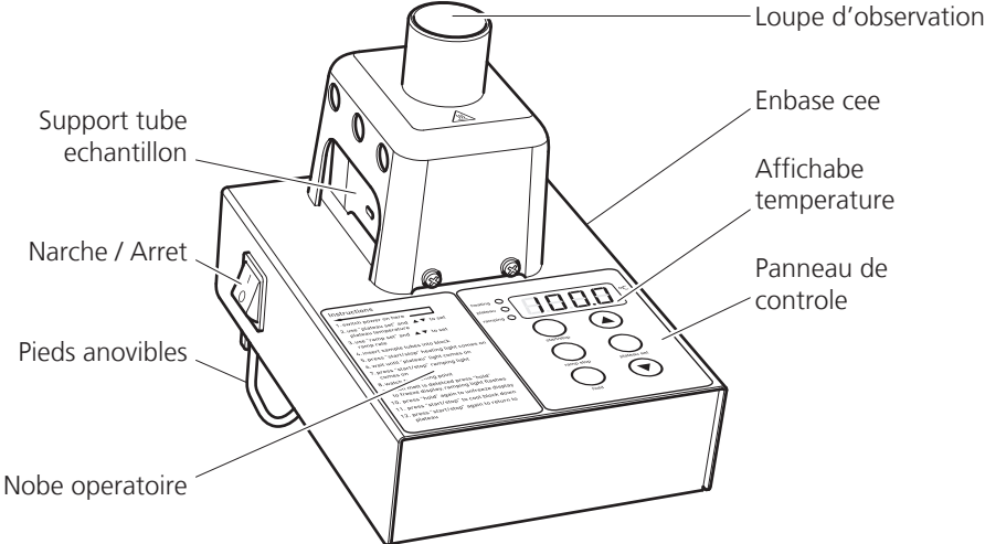
MP-200D Fascia
